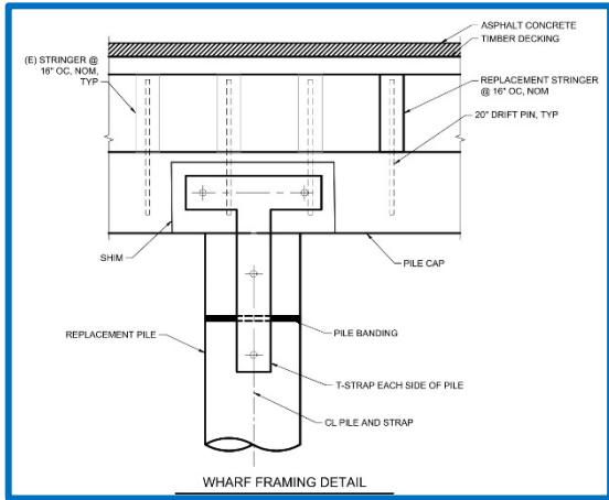
Wharf framing detail.
