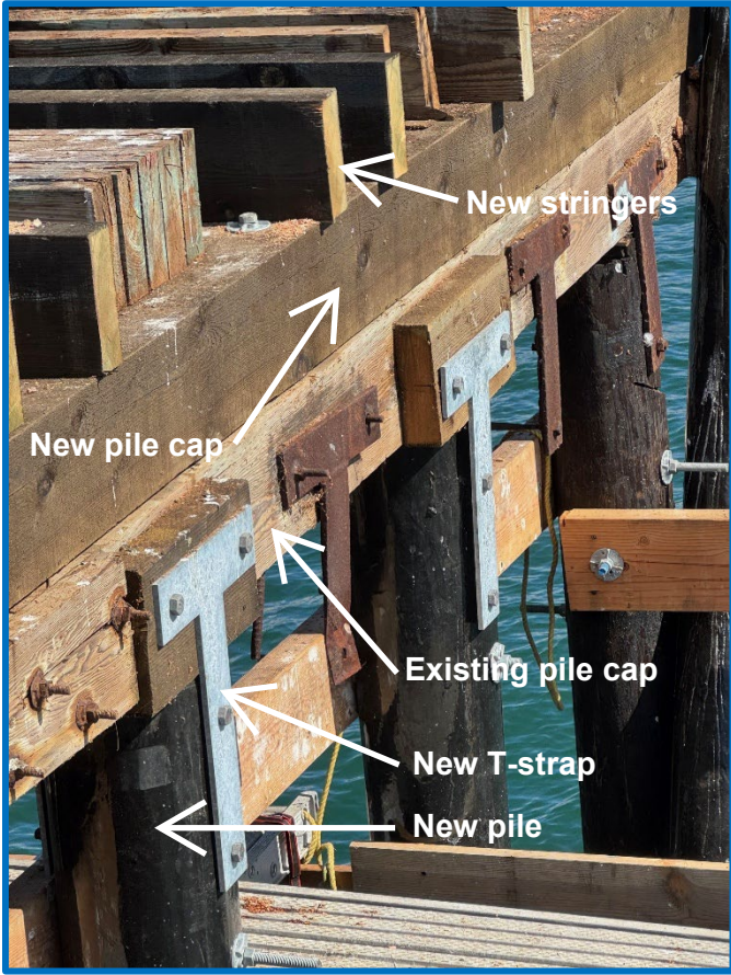
New T-straps connecting new piles to pile caps.
