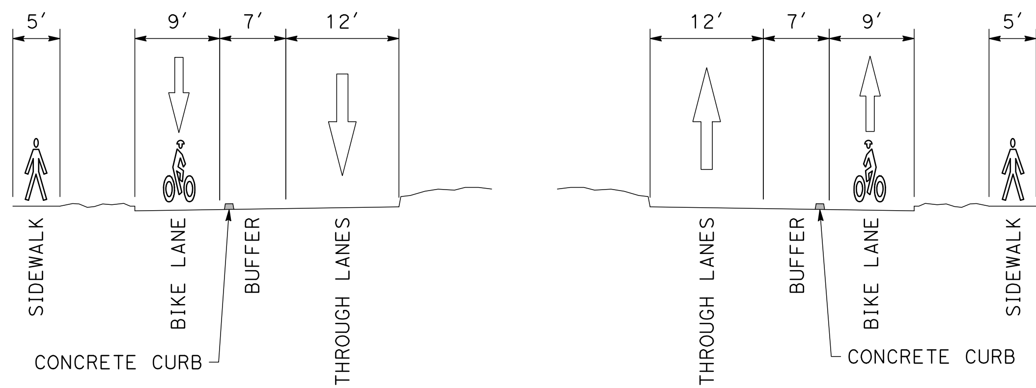
SECTION H-H
