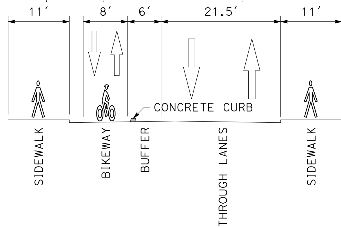
SECTION F-F
