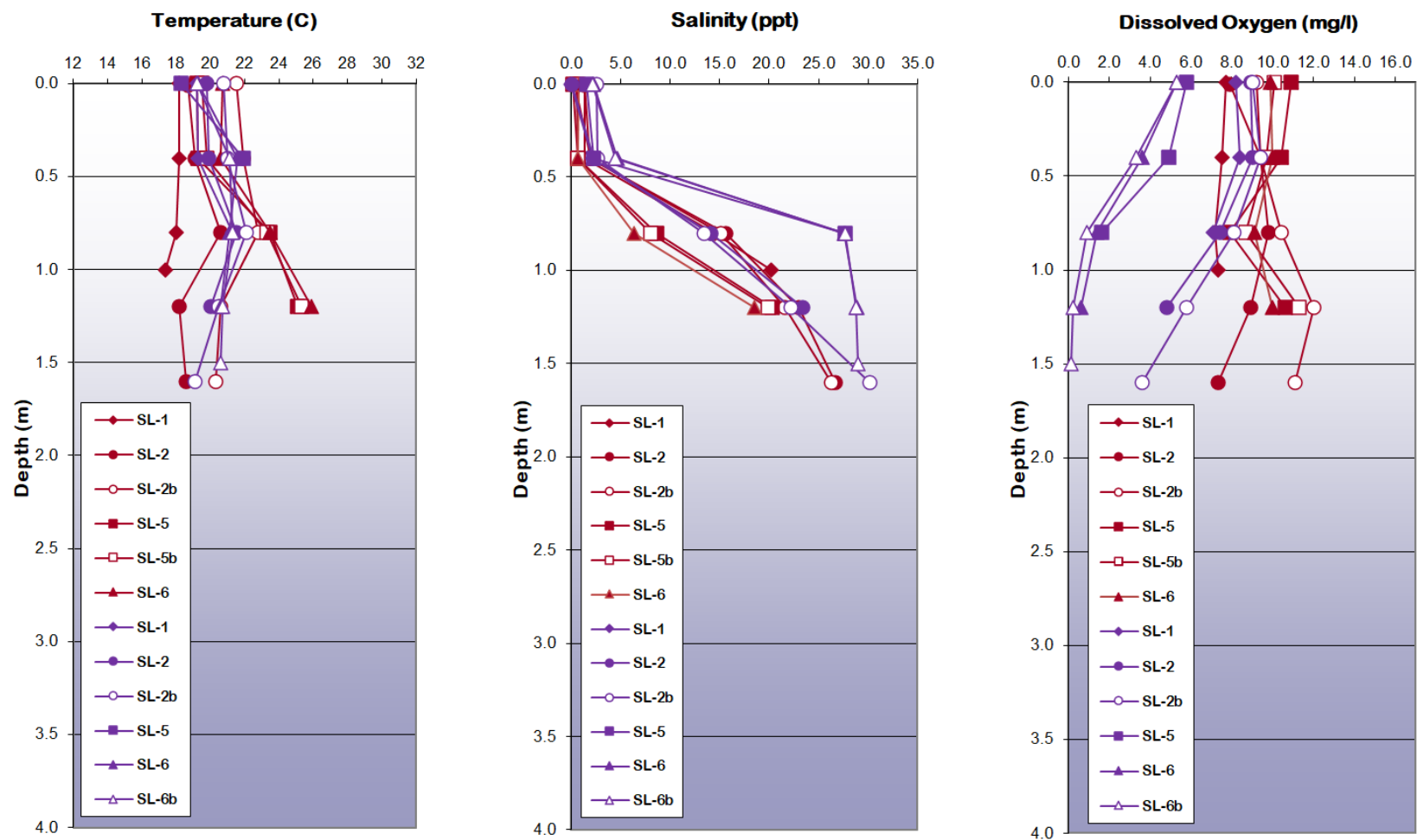
Figure 17. Depth profiles of water quality parameters in the San Lorenzo River Lagoon during June. Profiles plotted in red are June 7-8; profiles in blue are June 9-10
